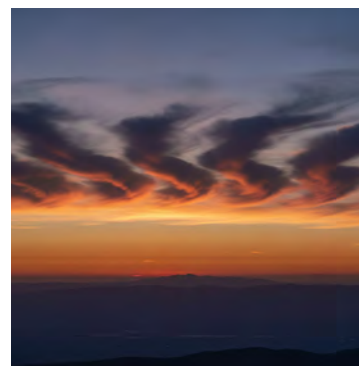
Kelvin-Helmholtz-Wolke (Fluctus)
